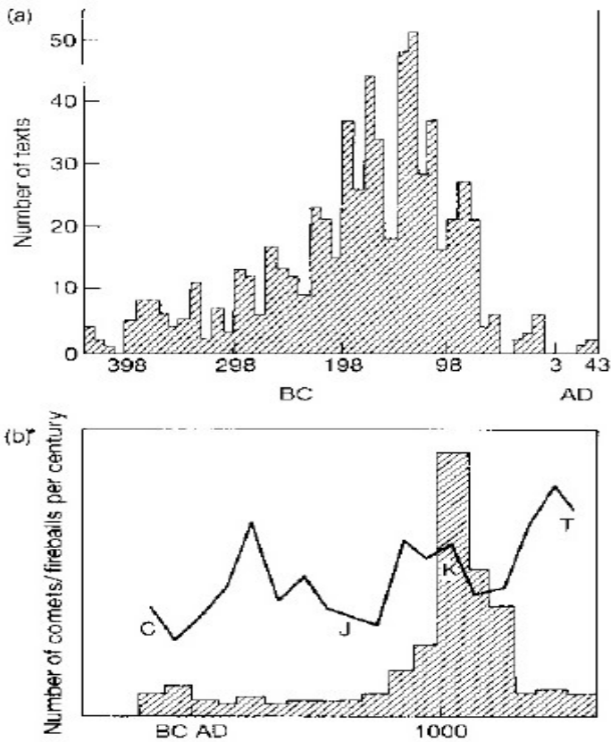
Figure 4. diagrams illustrating the apparent enhancement of fireball activity (a) during the late Babylonian period (based on recovered ephemerides and monthly records on cuneiform tablets); and (b) during the Chinese Tang dynasty (based on recorded fireball and comet observations, where the commonest fireball radiants during the eleventh-century peak arise from the Taurid meteor stream). In interpreting these apparent surges account must be taken of variation in the attention given to the sky by astronomers at different epochs (see also The Origin of Comets by M.E. Bailey and the authors). Also relevant is the location of astronomers, the increasing trend in the observed number of comets per century apparently reflecting the spread of professional astronomical practice from the Chinese (C) to the Japanese (J) and Koreans (K) before the introduction of the telescope (T).
