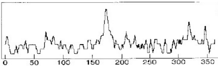
Figure 6. Diagram showing the average number of meteoroids striking the Moon on each day of the year over the period 1972-76, as recorded with seismometers left by the Apollo astronauts. The conspicuous peak at the end of June represents the flux over a few days in 1975 due to a swarm of more massive meteoroids coinciding with the Beta Taurid stream.
