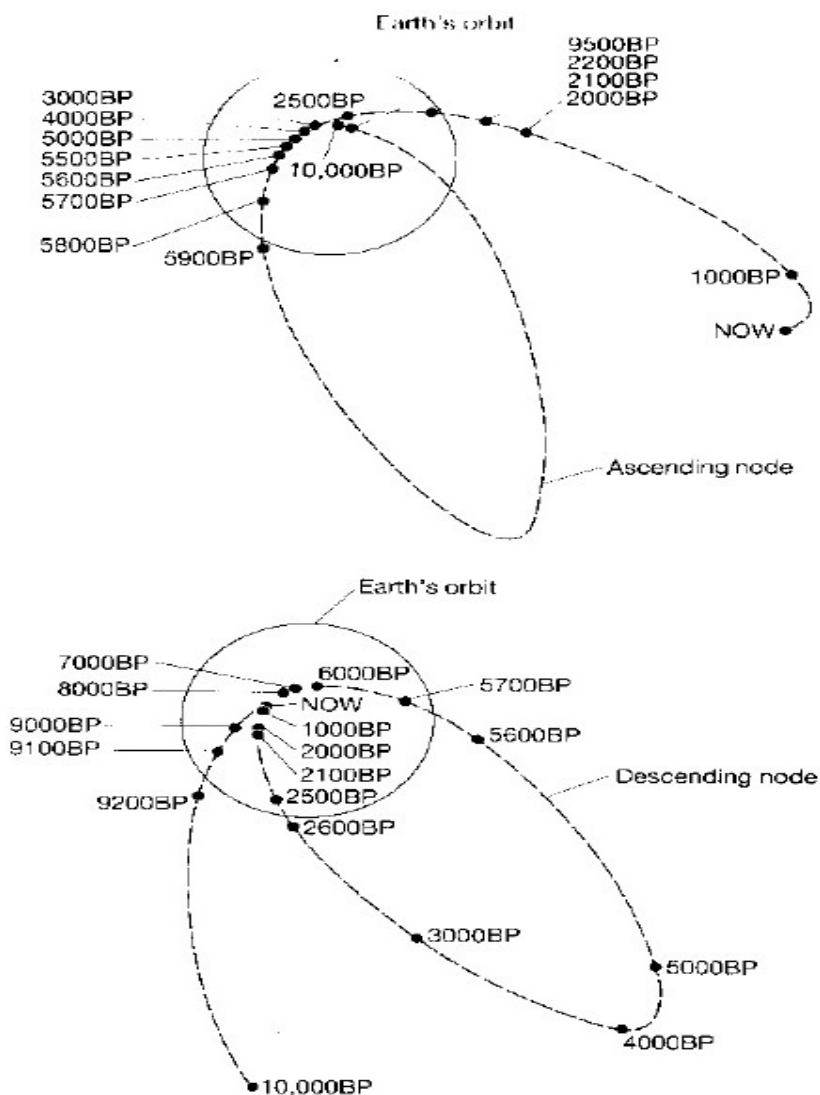
Figure 9. Intersection points (nodes) of Comet Encke's orbit with the plane containing the Earth's orbit, at various dates before the present (BP). During the first millennium BC up to the time of Christ, the orbit of the comet or that of its associated dust trail would have intersected that of the Earth, leading at this time to annual fireball storms of amazing intensity.
