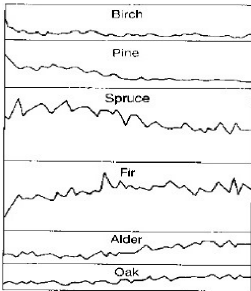
Figure 21. Fossil pollen record in a European peat bog, after G. Woillard. Time moves from right to left and a 300-year period is covered. The extreme left of the record shows a sudden but lasting change in forest composition, from predominately fir to a colder birch and pine. This sudden cooling of the European climate might have been caused by a stratospheric dusting, from impact or meteoric dust, causing a climatic instability and a change in ocean circulation patterns.
