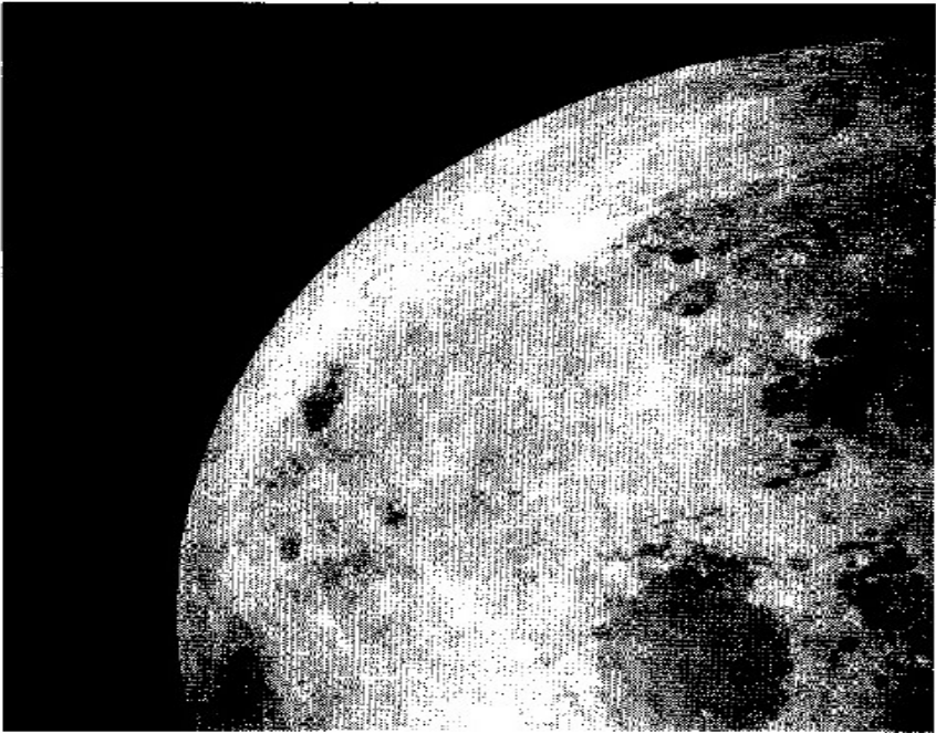
Plate 16. The Giordano Bruno crater on the Moon, photographed during the ill-fated Apollo 13 mission. Note the strikingly vivid (i.e. fresh) rays indicative of recent formation (by kind permission of the Johnson Space Center Mapping Science Laboratory ).
