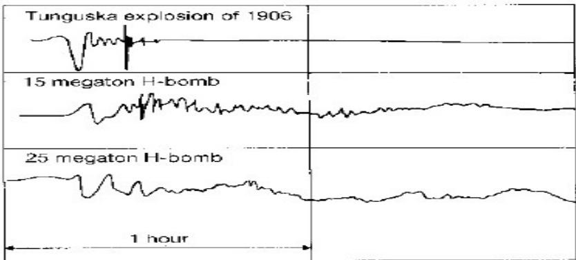
Figure 8. Pressure waves from the Tunguska explosion detected in south-east England 5720 km for the impact. For comparison, pressure waves form hydrogen bomb explosions are shown also: Bikini to barograph at Aspendale 5920 km, and Novaya Zemlaya to Aspendale 14000 km. from this an impact energy of about 30 megatons can be inferred. From E.L.Deacon (note 84).
