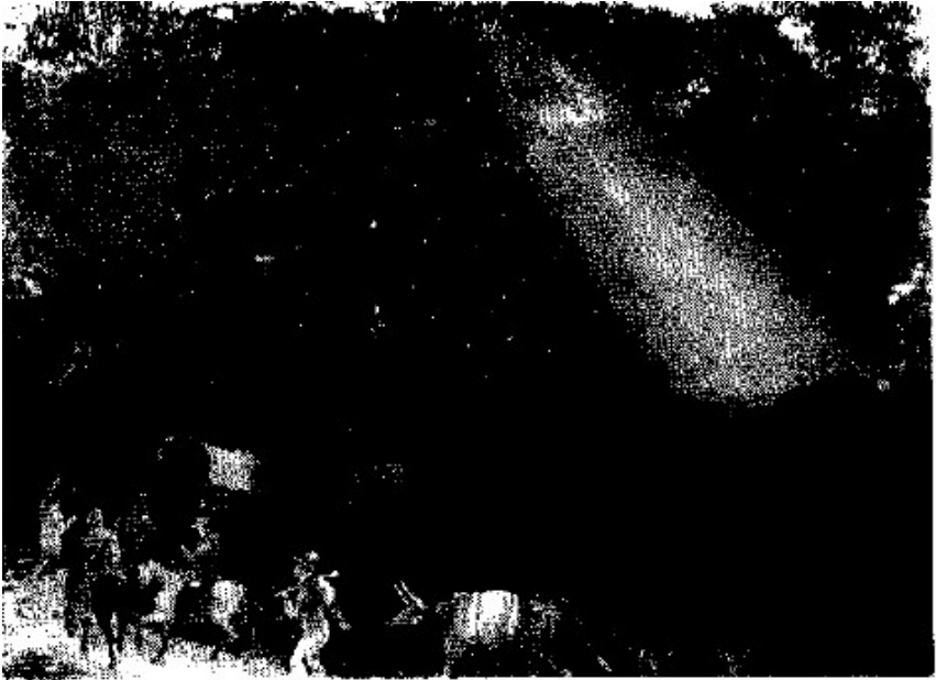
Plate 6. Visible debris from Encke's Comet or its progenitor: the Zodiacal Light from South Africa, 7 June 1843, as drawn by the Edinburgh astronomer Charles Piazzi Smyth. The light is aligned along the path of the zodiacal constellations, and was the track along which, in remote antiquity, active comets from the Encke material moved (by kind permission of Don Africana Library, Durban, South Africa).
