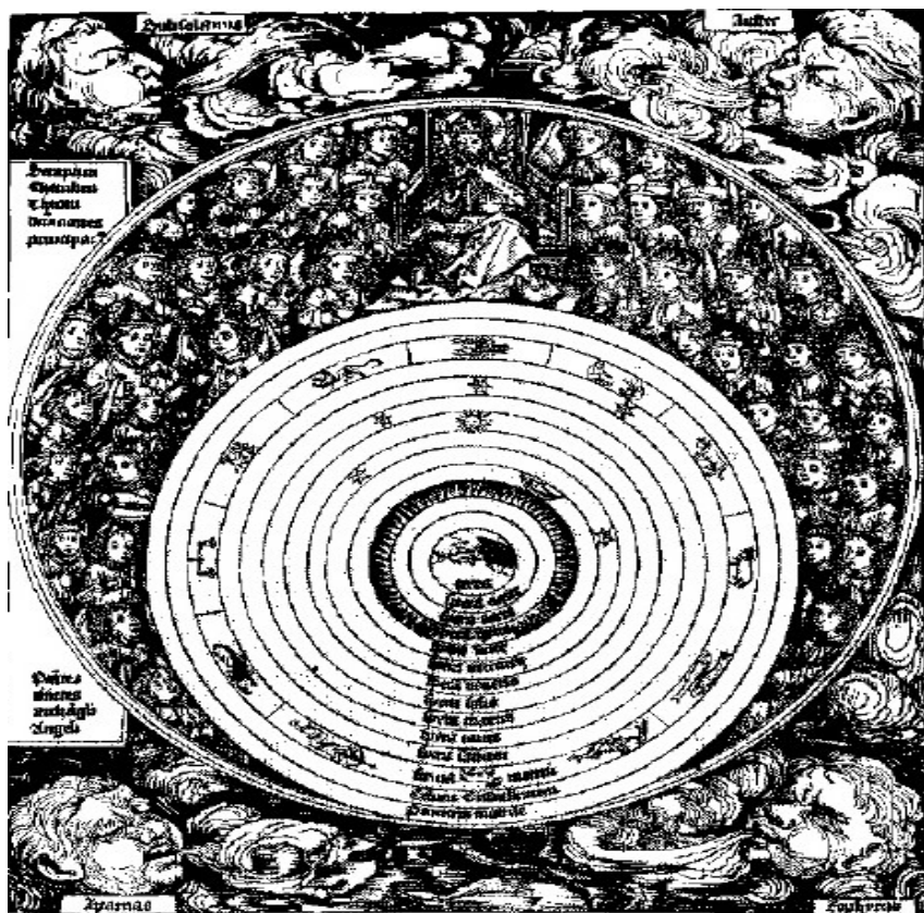
Plate 8. The Aristotelian planetary system as represented by the Nurnberg Chronicle of 1493 (reproduced by permission of Sotheby's, London). The Earth (terra) resides at the centre of a series of concentric spheres representing the other three basic elements (water, air, fire), all of which, according to Aristotle as he was interpreted by medieval philosophers, are associated with their particular ideal levels. Beyond that are the crystalline spheres to which are attached the celestial bodies: first the Moon, then Mercury and Venus, the Sun and the outer three planets, Mars, Jupiter and Saturn. Next comes the sphere of the zodiac and then the sphere of the fixed stars in countless numbers. The penultimate sphere is Aristotle's Prime Mover', whilst the final sphere is the domain of God and the Heavenly Host. This was to remain the popular image of the cosmos long after the investigations of Kepler, Copernicus and Galileo had posited a quite different order.
