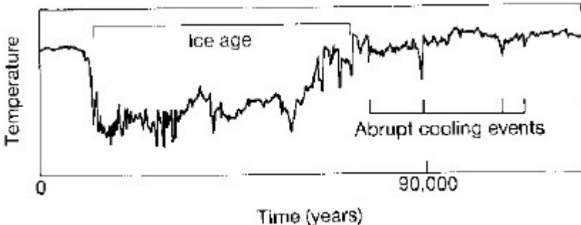
Figure 20. An early temperature record of the last major glaciations, after Dansgaard and his colleagues, from a study of cores extracted from the Greenland ice cap. According to the theory described here, this is essentially a record of stratospheric dusting due to material from the progressively disintegrating Comet Encke progenitor. Note the rapid flickering, the suddenness of onset of individual ‘flickers’, each a cosmic winter, and the rapidity with which the ice age ended. These sudden changes are not consistent with slow orbital and polar variations as the prime movers, but are expected on the giant comet picture.
