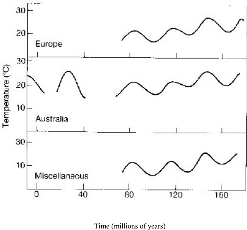
Figure 12. A 30-million-year cycle in global temperature, claimed by Dorman in 1968 using the proportion of 'heavy carbon' in fossil shells as a thermometer. Little weight should be given to the 'cycles' on the left due to the sparseness of the data on which they were based.
