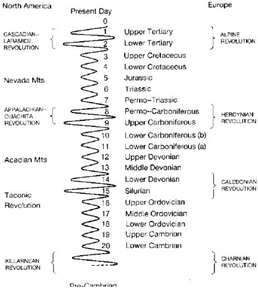
Figure 11. Sea level cycles of 30 and 250 million years, claimed by Arthur Holmes in 1927 and correlated by him with periodic geological disturbances (line drawing published by Benn, London). Although this diagram is qualitative and was drawn long before plate-tectonic theory, it anticipates much recent, quantitative research on geological cycles.
