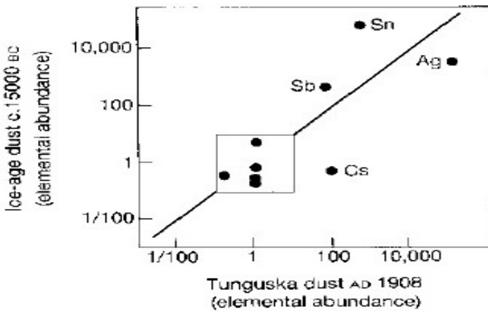
Figure 23. (a) Nickel-iridium ratio for small dust particles laid down on Greenland over the period 19700-14200 BP (filled circles), and from microparticles found at the site of the Tunguska explosion of AD 1908. Both these elements are found in cosmic particles. The good fit of both sources on to the line may imply a common progenitor body, as anticipated from the theory. (b) Comparison of abundances of various elements from the Greenland ice particles and from the Tunguska particles. Material in the box had the 'universal composition' found in unprocessed astronomical bodies. Both dust deposits have identical anomalies relative to the mix – large overabundances of tin (Sn), silver (Ag), Caesium (Cs) and antimony (Sb) – again consistent with a common source, and hence a cometary origin of the Greenland dust.
