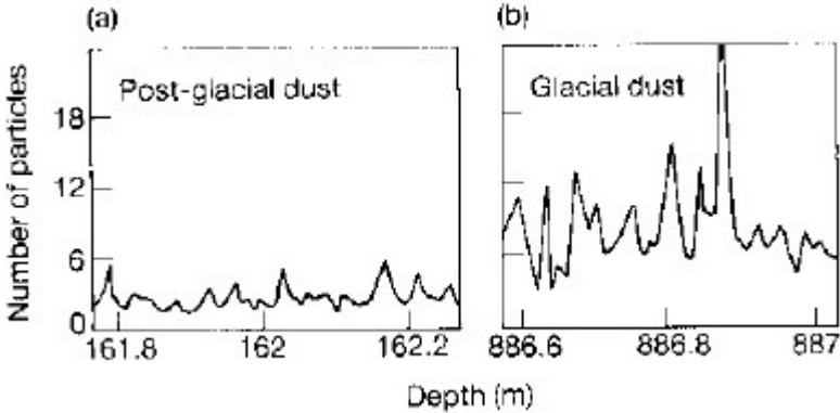
Figure 22. Typical depositions of sub-micron dust particles in polar regions during glacial and post-glacial times (due to Thompson and Mosley-Thompson, 'Microparticle concentration variations' ). Note the enhanced dust levels during the last ice age. A significant proportion of this material seems to be cometary in origin.
