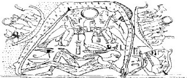
Plate 5. In the writings of early Greek natural philosophers, the heavenly path of the Sun was associated with the Milky Way. A similar personification of the Sun's path is found in ancient Egypt where it is represented by (a) the star-spangled cow-goddess Hathor, later Isis (line drawing reproduced by permission of Weidenfeld & Nicolson), or by the similarly decorated mother-goddess Nut, not bearing (b) or bearing (c) the solar barque as the case may be (line drawings reproduced by permission of Crossroad/Continuum).
