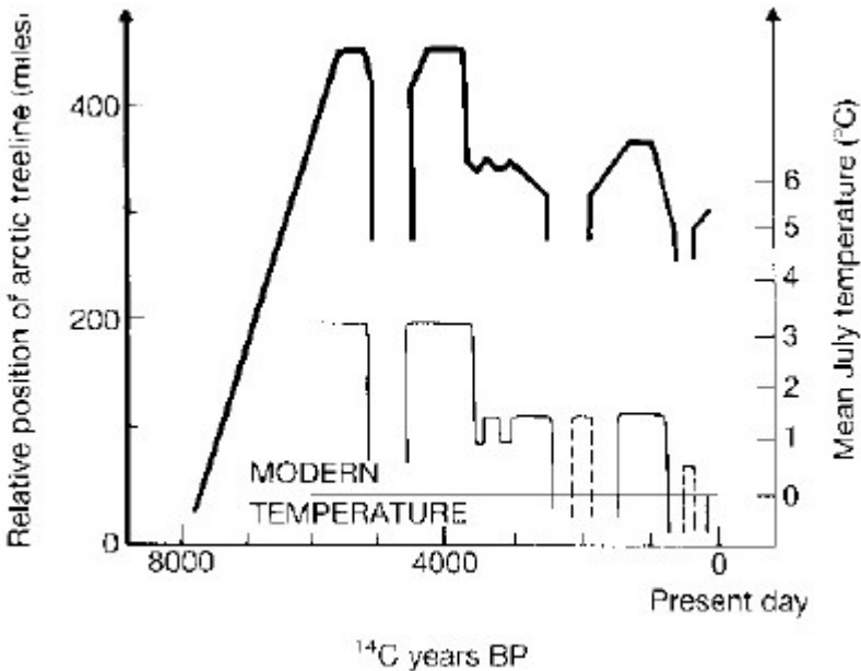
Figure 2. Mean summer temperatures (global average relative to its present day value) based on the movements of the Arctic treeline during the last 7,000 years (reproduced from The Little Ice Age by J. Grove). The sustained amelioration during the period 6000-1500 BC corresponds to the recognized climatic optimum of the Holocene period, whilst the broken lines indicate possible brief ameliorations due to a reduced incidence of atmospheric dust veils, as indicated by acidity peaks in Greenland ice cores and frosted tree rings.
