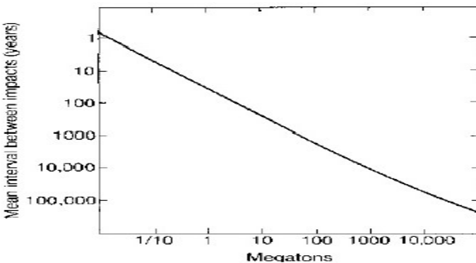
Figure 19. Baseline rate for impacts of various energies on the Earth, after E.M. Shoemaker. Based on the size distribution of small craters on the Moon.
