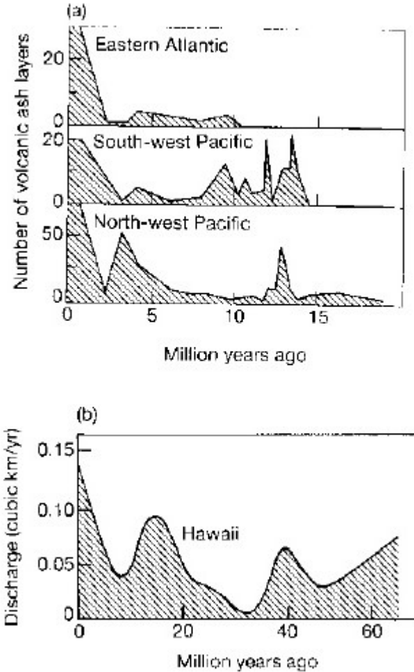
Figure 18. Outpourings of lava from various oceanic sites. Peaks in the output can be seen at around 40 million years ago, some 15-10 million years ago, and within the last few million years. These epochs are consistent with the peaks in the cratering record
