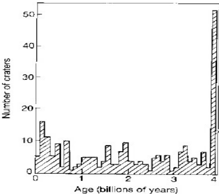
Figure 17. Lunar cratering history, from 3.9 billion years ago to the present (due to Baldwin). The average impact rate has been relatively constant although surges lasting not more than 50-100 million years of uncertain date are also present. A huge reservoir of potential impactors is implied, along with a relatively steady input mechanism. The Galaxy may both replenish and disturb the cloud of comets surrounding the Solar System. The high impact rate 3-9 Byr ago and even higher rates earlier are ascribed to the mopping up of debris left over from the origin of the planetary system, and are apparently unrelated to the cratering history since.
