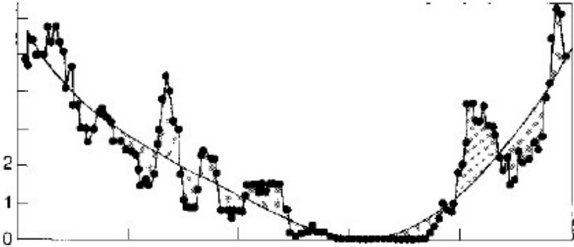
Figure 15. Frequency with which the north and south magnetic poles of the Earth interchange, after K.M.Creer and P.C.Pal. in this more nearly complete geological record a variable 15/30-million-year cycle is clearly seen superimposed on longer-term trends.
