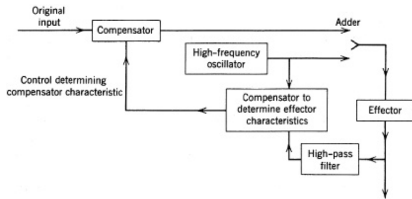
Figure 0.3 Feedback system 17
