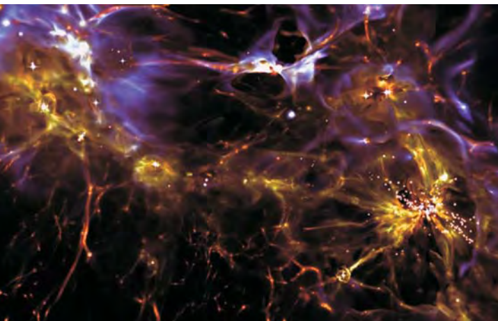
Figure 5. Galaxy seeds. The earliest supernovae propelled material to great distances through the intergalactic medium. Gravitational interactions caused that material to collect into galaxies. In this simulation, a number of small galaxies are visible in yellow. The largest of those, visible to the lower right, has a mass only 1/5000 that of the Milky Way. Hundreds of regions such as those shown here will combine over a few billion years to form galaxies like our own. The reddish areas are regions in which stars have not yet formed. (Simulation by John Wise, Tom Abel, and Michael Norman; image by Ralf Kaehler and Tom Abel.)
