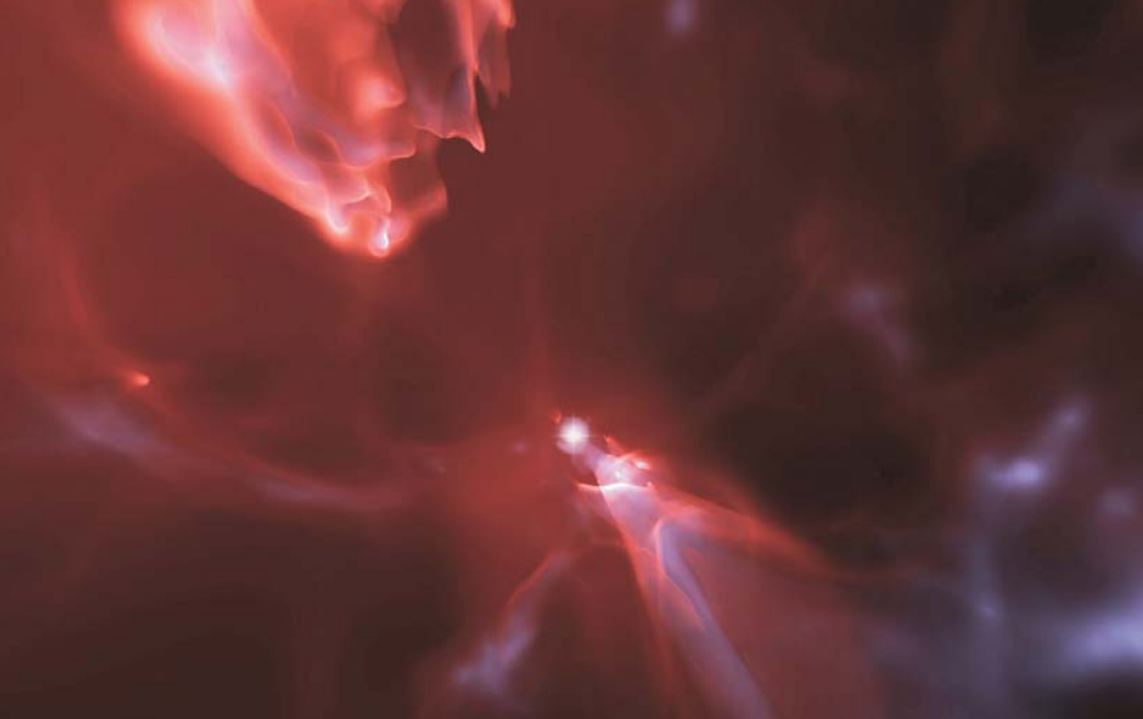
Figure 4. Blown away. Massive stars are hot and intensely bright. The radiation they emit ionizes hydrogen out to thousands of light-years, and the associated pressure clears material away from the star. In the simulation shown here, a bright star sits roughly in the center of the frame. Except for a small angular region to its lower right, the star has largely blown away its surroundings, which appear darker in the image. If the star is massive enough, it may end its life as a black hole in an environment where there is little to accrete. (Simulation by John Wise and Tom Abel; image by Ralf Kaehler and Tom Abel.)
