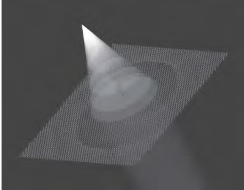
Fig. 7.2. Silicon nanopillars arranged in a hexagonal pattern create a “metasurface” that generates and focuses radially polarized light. Think solar simulator.
