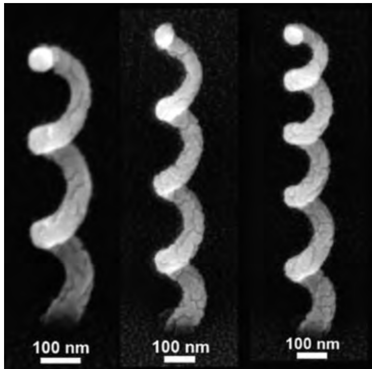
Fig. 9.1. Helix-shaped nano-antennas produced in an electron microscope by direct electron-beam writing and created from the Lyme spirochete Borellia burgdorferi . Helmholtz Zentrum Berlin, image © HZB
