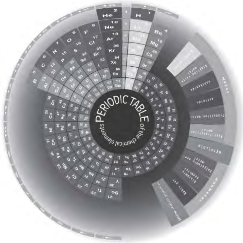
Fig. 2.3. The periodic table of elements. Image ID 47259048 by Danielz1 | Dreamstime.com
