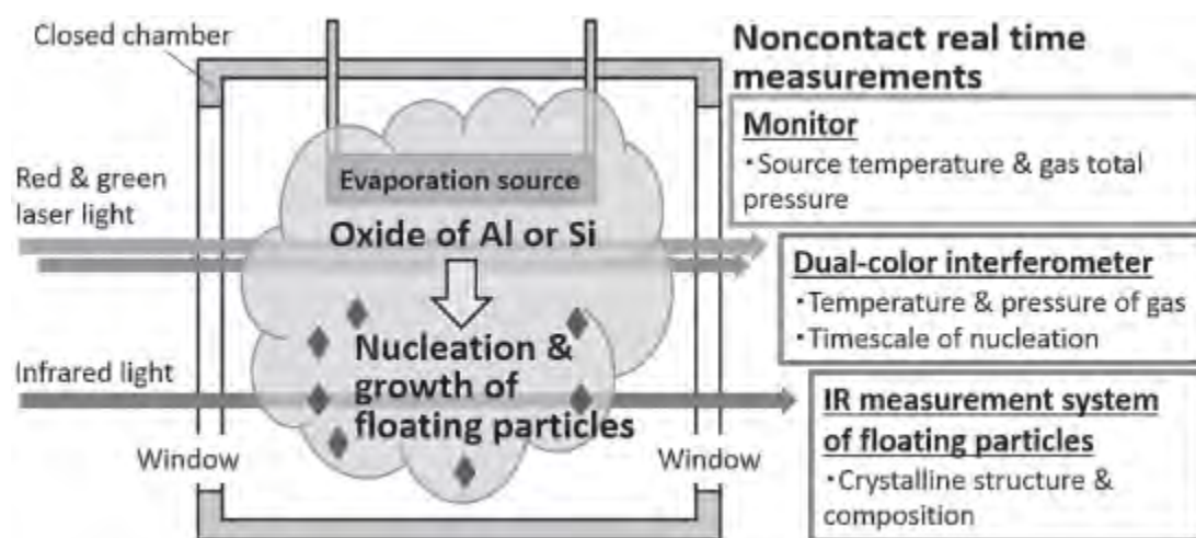
Fig. 2.2. Nucleation and growth of oxide nanoparticles, aka star “crumbs.” Hokkaido University: “We identified the initial conditions required to form nanoparticles, the basic building blocks of earth-like planets. In particular, we searched for conditions where nucleation of oxidized aluminum and silica could easily occur, and we identified the first nanoparticles which govern the evolution of cosmic dust.”
