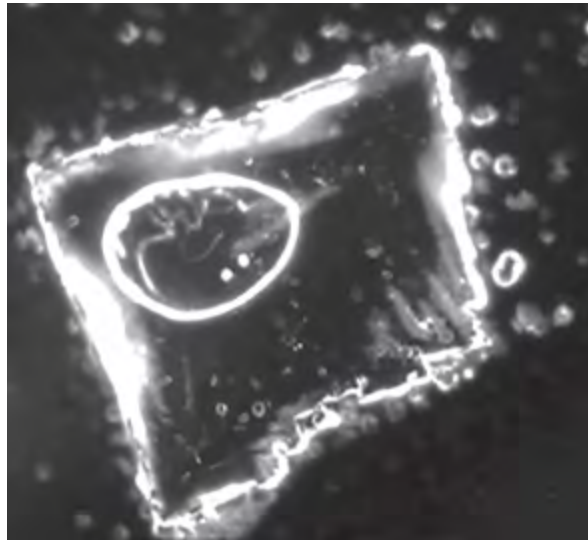
Fig. 8.2. Complex crystal structure that has formed from a drop of rainwater after a period of aerial spraying. This crystal can be seen at the bottom of the circular image above.
