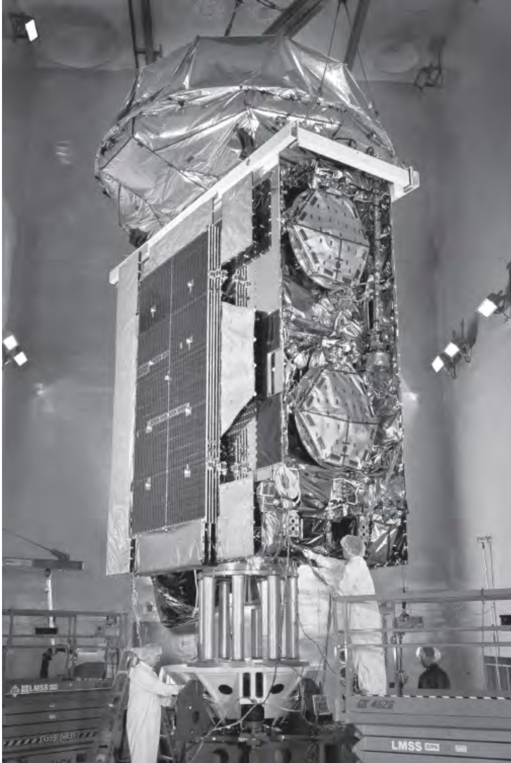
Fig. 3.2. MUOS satellite (Mobile User Objective System). Satellites do not necessarily look as impressive as their tasks indicate they are. Developed by Lockheed Martin for the U.S. Navy, MUOS is an ultrahigh frequency (UHF) SATCOM system of four orbiting satellites and four relay ground stations of the Space Fence infrastructure. Note the hexagons. MUOS looks like the Wicker Man in the film The Wicker Man (1973, 2006).
