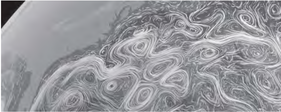
Fig. 1.5. Gulf Stream NASA, Florida-Carolinas coast, U.S.A. NASA/Goddard Space Flight Center Scientific Visualization Studio
