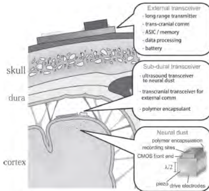
Fig. 3.3. Neural dust—see how it's engineered.
