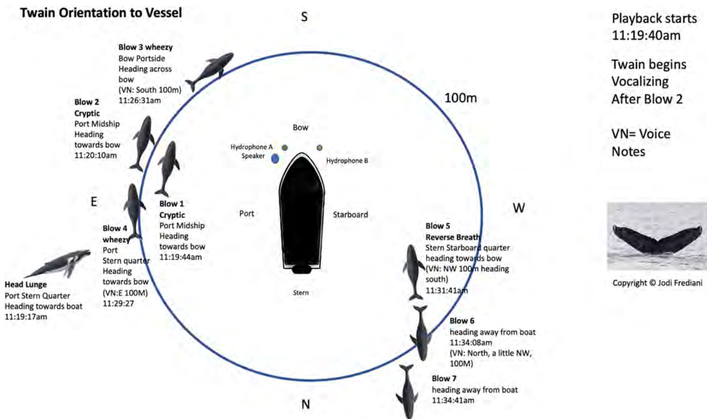
Figure 2 Twain's surface tracking and behavior during the playback phase of the trial (see Fig. 1B). Whale image with text indicates position and behavior of Twain during playback trial. Boat image represents the R/V Glacier Seal . Hydrophones and speaker placement indicated. Fluke ID shot of Twain during the interaction.
