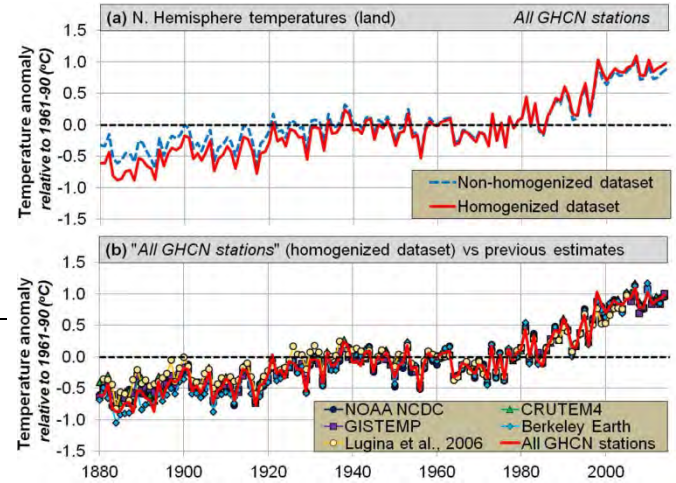
Figure 20. (a) Comparison of gridded mean temperature trends for all Northern Hemisphere stations in the Global Historical Climatology Network (GHCN) homogenized and non-homogenized datasets. (b) Comparison of the homogenized version to five other recent estimates, which were downloaded from their respective websites on 18 th March 2015: CRUTEM4 ( http://www.cru.uea.ac.uk/cru/data/temperature/ ); NOAA NCDC ( http://www.ncdc.noaa.gov/monitoring-references/faq/anomalies.php ); GISTEMP ( http://data.giss.nasa.gov/gistemp/ ); Lugina et al., 2006 ( http://cdiac.ornl.gov/trends/temp/lugina/lugina.html ); Berkeley Earth ( http://berkeleearth.lbl.gov/regions/northern-hemisphere ).
