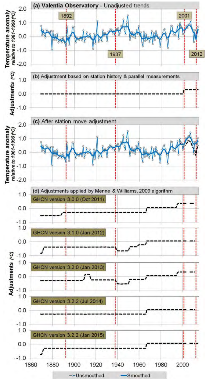
Figure 15. (a) Valentia Observatory record before adjustment. (b) Record adjustment to account for 2001 station move. (c) Record after adjustment. (d) Adjustments generated by the Menne & Williams, 2009 algorithm. Red dashed lines indicate station history events.
