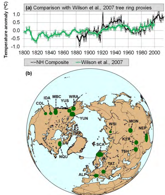
Figure 24. (a) Comparison with Wilson et al. (2007)'s extra-tropical Northern Hemisphere tree-ring-based temperature proxy reconstruction. (b) Approximate location of the 15 tree ring chronologies used by Wilson et al. (2007) for their extra-tropical temperature proxy reconstruction (adapted from their Figure 2). For explanations of the labels, see Wilson et al. (2007).
