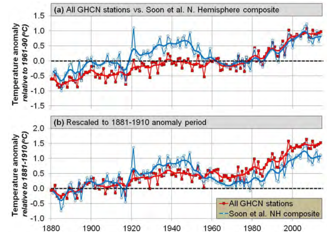
Figure 21. Comparison of our Northern Hemisphere composite to the equivalent estimate using all Northern Hemisphere stations in the Global Historical Climatology Network (GHCN) homogenized dataset. Temperatures relative to (a) 1961-1990 and (b) 1881-1910.
