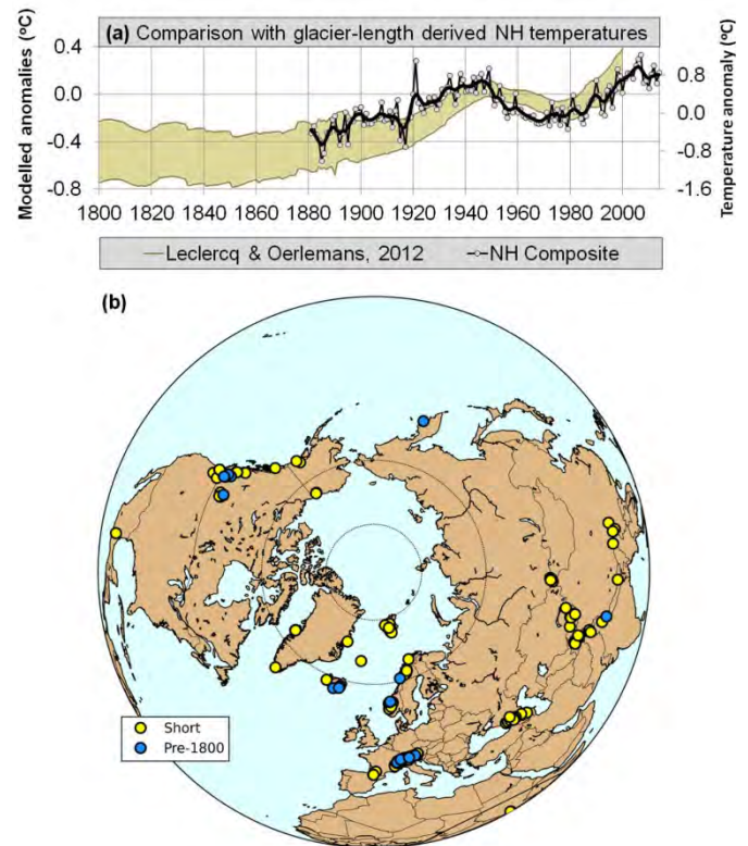
Figure 23. (a) Comparison with Leclercq & Oerlemans, 2012’s glacier length record derived Northern Hemisphere temperature reconstruction. The y-axis on the left corresponds to the modelled temperature anomalies of the reconstruction and the y-axis on the right corresponds to our composite. (b) Location of glaciers used by Leclercq & Oerlemans, 2012 for their Northern Hemisphere glacier length record derived temperature reconstruction. Blue circles indicate the locations of the 24 glaciers (out of 247) with data before 1800.
