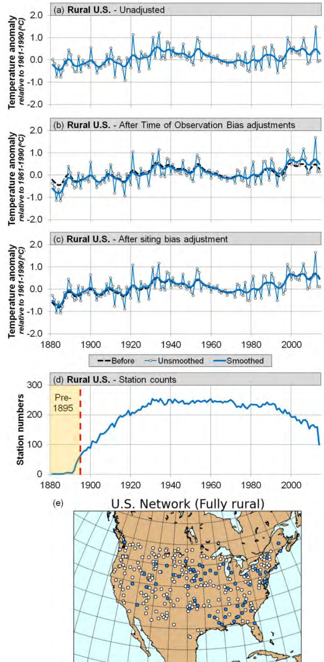
Figure 14. (a-c) Rural U.S. temperature trends before (black dashed lines) and after various adjustments to account for non-climatic biases. (d) Stations used for each year. (e) Locations of fully rural U.S. Historical Climatology Network (USHCN) stations used. Filled blue circles indicate the locations of those stations with data before 1895.
