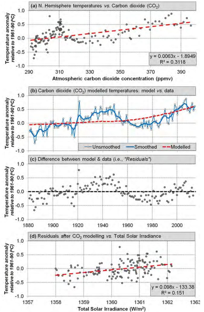
Figure 30. As for Figure 28, but fitting using measured changes in atmospheric carbon dioxide ( \text{CO}_2 ).
