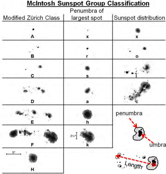
Figure 6. The three component McIntosh classification system for sunspot groups. Adapted from Figure 1 of McIntosh (1990).
