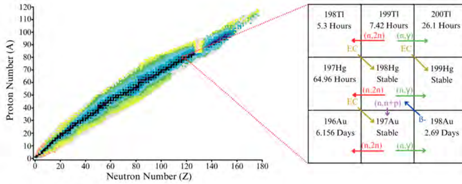
Fig. 1: Table of nuclides (from NuDat.[16]) with a zoomed view of the region of interest. Arrows show how neutron-driven reactions and radioactive decay direct transmutation. EC stands for electron capture.
